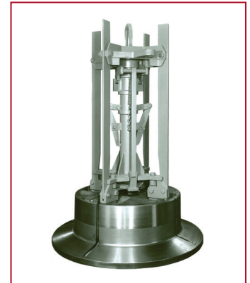
Stripper Block
